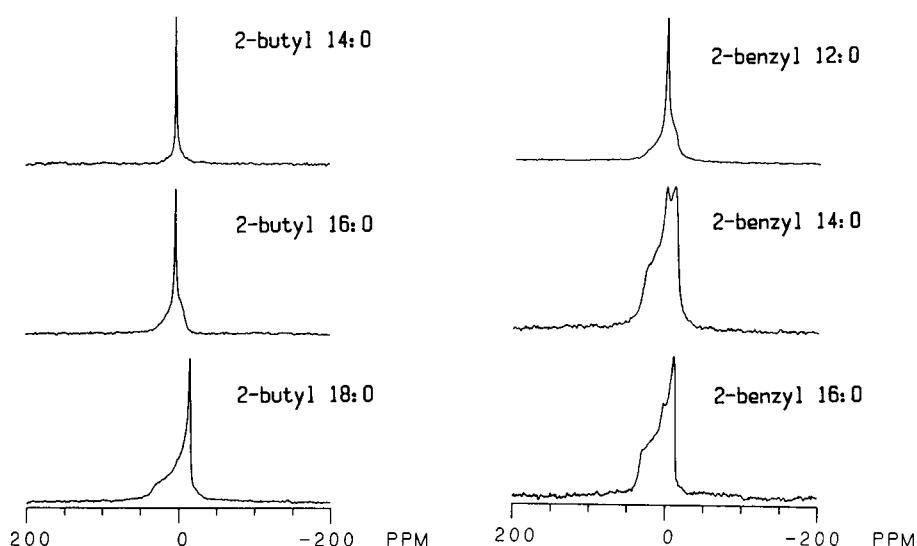
FIGURE 7 Proton-decoupled ^{31}\text{P} -NMR spectra of di-( dl )-2-butyl- (left panel) and di-( dl )-2-benzyl-substituted analogues of the homologous series of normal saturated diacyl PCs. The spectra shown were all acquired at 85°C.
