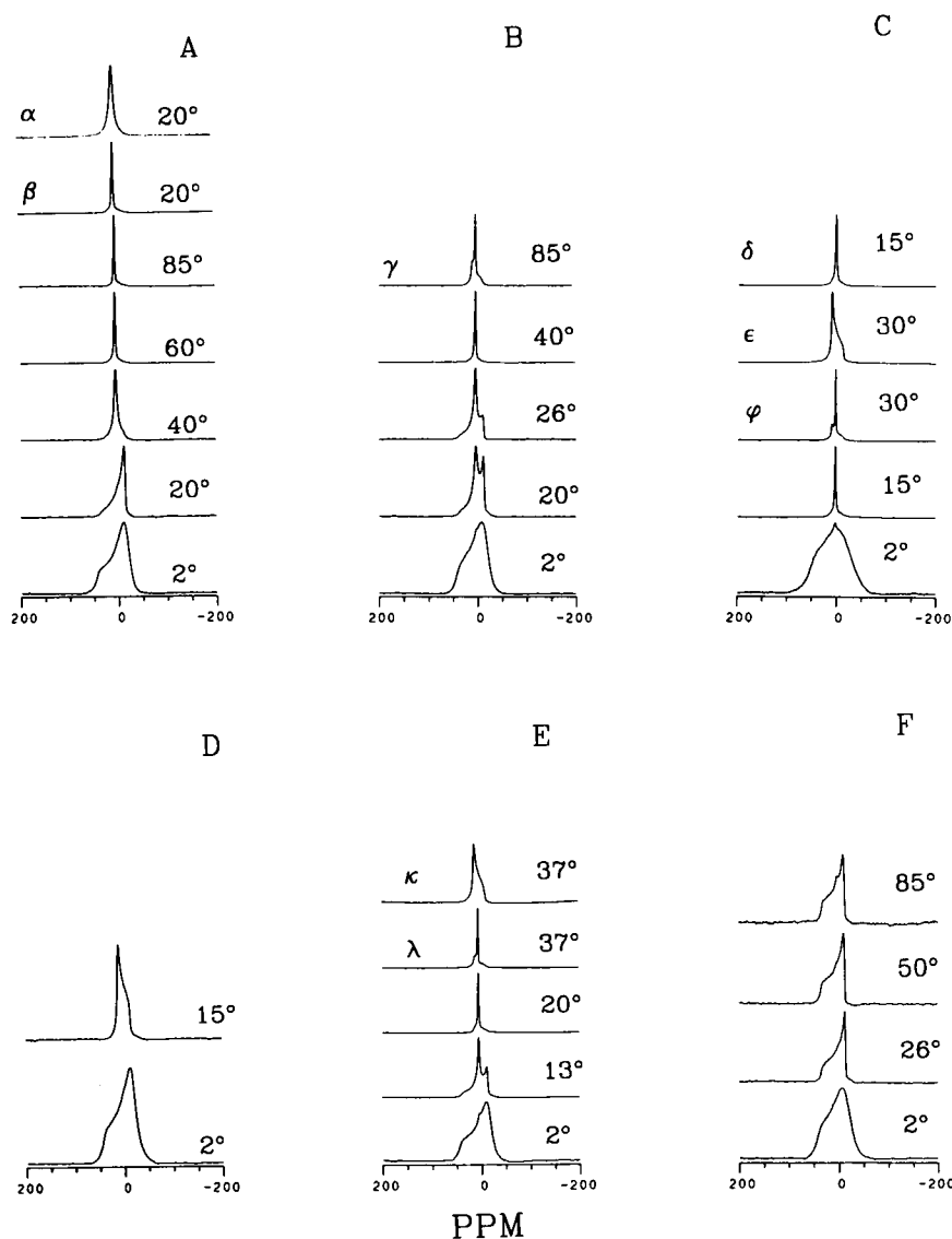
FIGURE 4 Proton decoupled ^{31}\text{P} -NMR spectra of (A) di-( dl )-2-(2-methyl butyl)-hexadecanoyl PC, (B) di-( dl )-2-(3-methyl butyl)-hexadecanoyl PC, (C) di-( dl )-2-(3, 3-dimethyl butyl)-hexadecanoyl PC, (D) di-( dl )-2-(cyclohexyl methyl)-hexadecanoyl PC, (E) di-( dl )-2-(2-ethyl butyl)-hexadecanoyl PC, and (F) di-( dl )-2-benzyl-hexadecanoyl PC. The spectra were obtained at the temperatures indicated and, unless otherwise stated, were acquired in a sequence corresponding to the heating mode of the DSC experiment. \alpha sample cooled from 40°C; \beta sample cooled from 85°C; \gamma sample quickly heated from 2°C; \delta sample cooled from 15°C; \epsilon sample quickly heated from 2°C; \varphi sample heated from 15°C; \kappa sample quickly heated from 2°C; and \lambda sample PC heated from 15°C.
